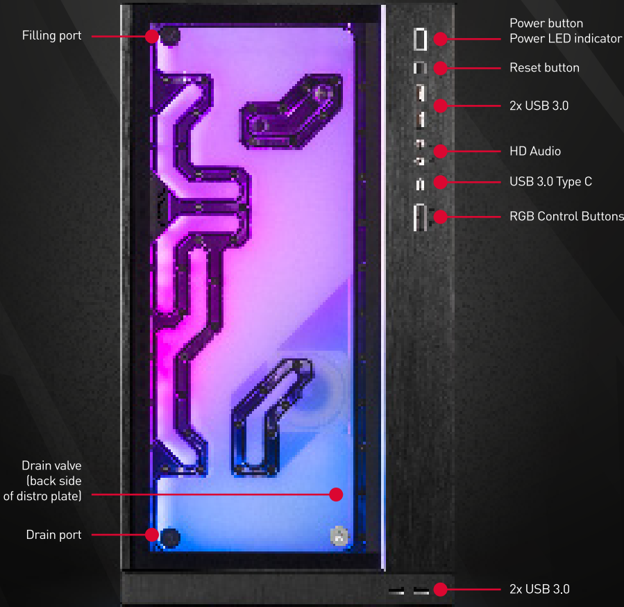
Port layout - Front
